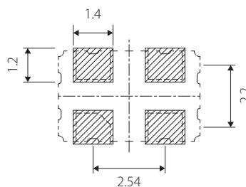
Land Pattern(REFERENCE)
