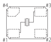
Land Pattern(REFERENCE)
